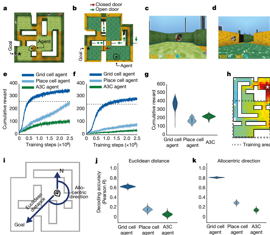
Fig. 3 | Navigation in challenging environments. a, b, Overhead view of multi-room environments goal-driven ( a ) and goal-doors (that is, with stochastic doors; b ). Goal (asterisk) and agent (head icon) locations are displayed. c, d, Agent views of a and b , respectively, showing red goal and closed black door. e, f, Agent training performance curves for a and b , respectively, and performance of human expert (dashed line). Performance is mean cumulative reward over 100 episodes. The grey band displays the 68% CI based on 5,000 bootstrapped samples. g, Distribution of test performance over 100 episodes, showing ability of agents to generalize to a larger version of the goal-doors environment, displayed with a violin
