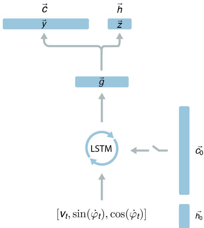
Extended Data Fig. 1 | Network architecture in the supervised learning experiment. The recurrent layer of the grid cell network is an LSTM with 128 hidden units. The recurrent layer receives as input the vector [v, \sin(\dot{\phi}), \cos(\dot{\phi})] . The initial cell state and hidden state of the LSTM, \vec{c}_0 and \vec{h}_0 , respectively, are initialized by computing a linear transformation of the ground truth place \vec{c}_0 and head-direction activity \vec{h}_0 at time 0. The output of the LSTM is followed by a linear layer on which dropout is applied. The output of the linear layer, \vec{g}_t , is linearly transformed and passed to two softmax functions that calculate the predicted head direction cell activity, \vec{z}_t , and place cell activity, \vec{y}_t . We found evidence of grid-like and head direction-like units in the linear layer activations \vec{g}_t .
