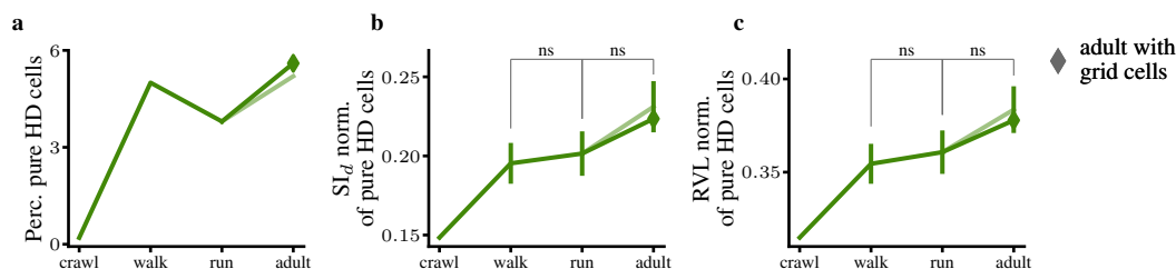
Figure A9: Pure directional selectivity emerges at the "walk" stage and remains stable thereafter. Diamonds indicate adult model trained with grid cell input. Non-significance was determined by one-sided pairwise Wilcoxon rank-sum tests (Wilcoxon, 1992) with Benjamini-Hochberg correction (Hollander et al., 2013) testing for increasing differences. a Percentage of RNN units classified as pure head direction (HD) cells – i.e., meeting only the criteria for directional selectivity. b Min-max normalised spatial information SI_d (mean \pm SEM) for polar maps of RNN units classified as pure HD cells. c Min-max normalised resultant vector length (RVL, mean \pm SEM) for polar maps of RNN units classified as pure HD cells.
