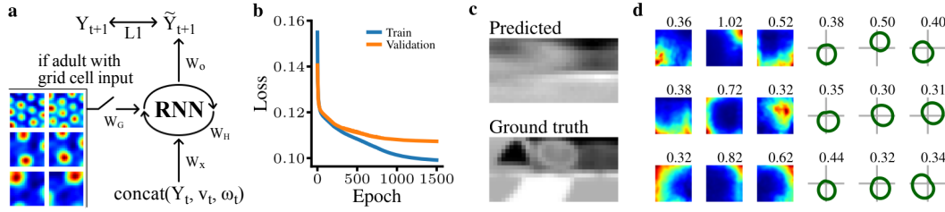
Figure 2: Recurrent neural network (RNN) model of hippocampal function. a RNN schematic. At each timestep t , the network received a concatenation of the agent’s visual input Y_t , velocity vector v_t , and rotational velocity \omega_t . For the adult locomotion stage, an additional variant was trained – where the hidden layer was initialised to a linear projection W_g of a population of grid cells at trajectory onset and every 90 timesteps. The predicted frame \tilde{Y}_{t+1} is decoded from the hidden state with a linear projection W_o and compared to the observed frame Y_{t+1} using the L1 distance. b,c,d RNN trained on simulated trajectories belonging to the adult locomotion stage. b Train (blue) and validation (orange) loss trends throughout training. c Example predicted frame (top) and its ground truth comparison (bottom), sampled from the validation set. d Subset of rate maps in (x,y) space (warmer colour indicate higher activity) of hidden units classified as place cells and corresponding SI_r values (left), and subset of polar maps in polar space of hidden units classified as head direction cells and corresponding SI_d values (right).
