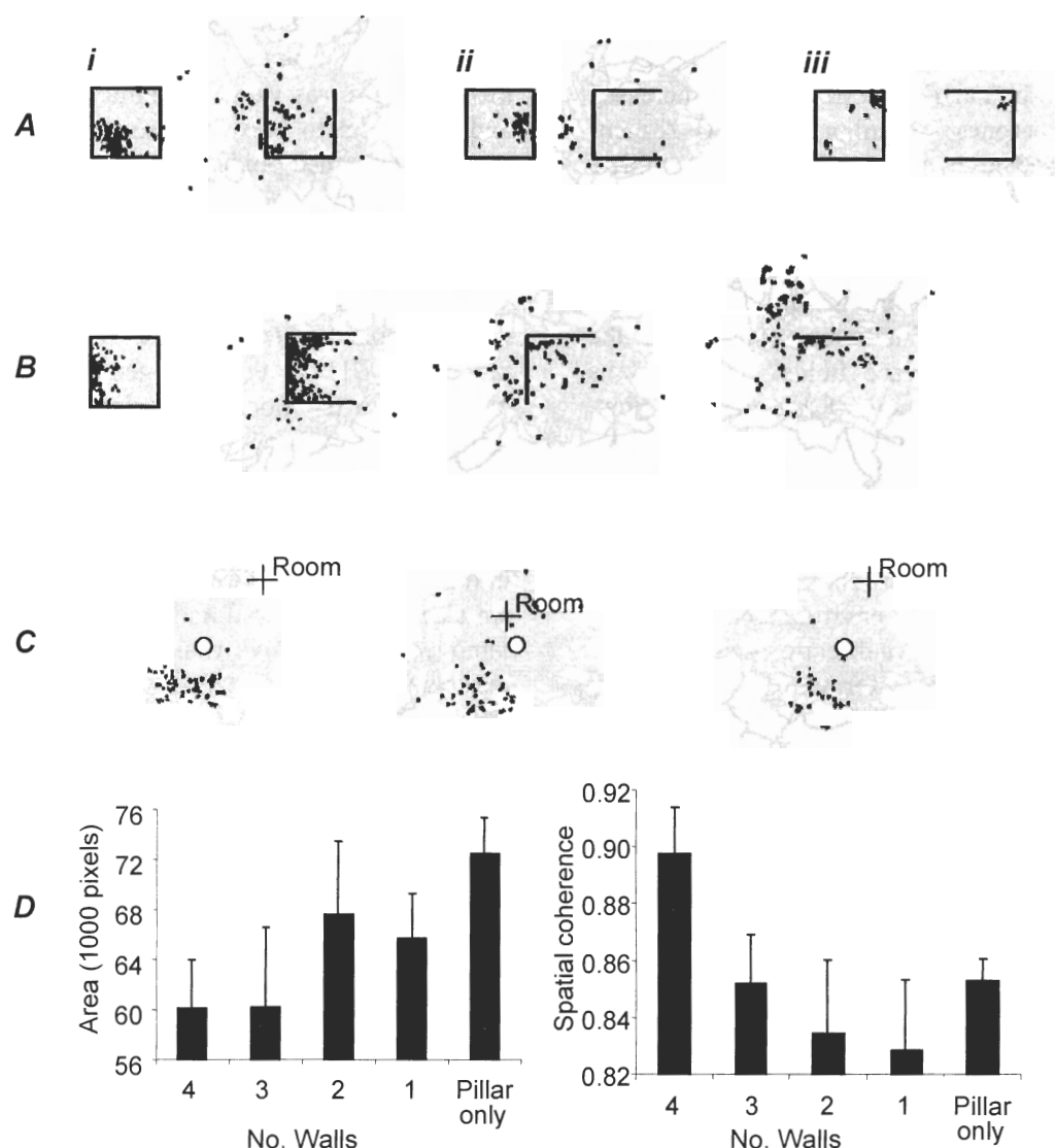
Fig. 3: Effect of wall removal on place cell firing. A. Effect of removing one wall. Three place cells are shown (i-iii). Plots show the locations at which spikes were fired (black squares) and the path of the rat (grey). Walls are shown as black lines. B. Effect of successive removal of walls on the firing of one place cell. Removal of the first wall produced limited change in the place field - three surrounding walls were sufficient to support spatial firing. Removal of the second wall, however, caused a profound breakdown in spatial firing. C. A rare place cell (one of two) with a coherent field in the pillar-only condition (after removal of all four walls). The location of the pillar is shown by 'o', a fixed point within the room is shown by '+Room'. D. Effect of successive wall removal on 17 place fields: they increase in area (left: kilo-pixels above half of the peak firing rate, entire camera view is 262 Kpix) and decrease in spatial coherence (right, see /60/, note that evenly scattered low firing produces high coherence).
