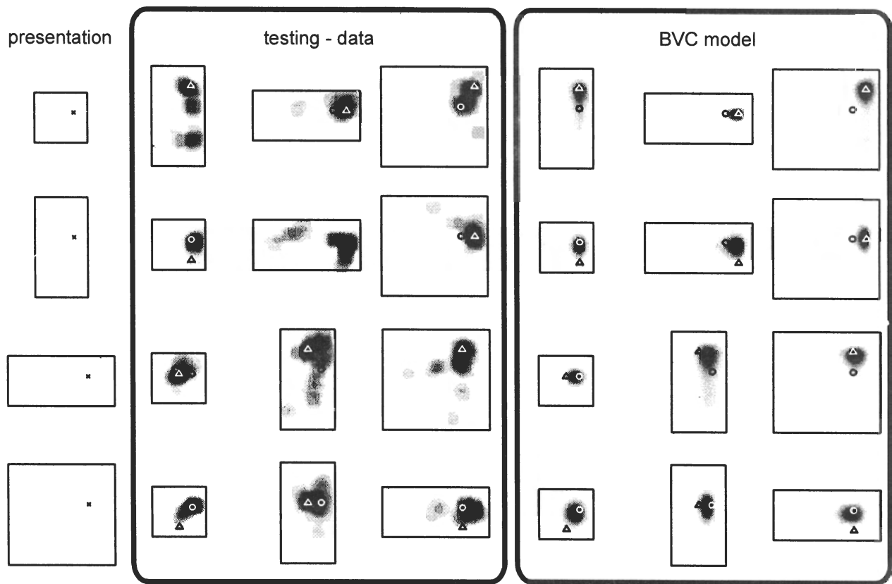
Fig. 6: Density of responses from a human spatial memory task ('testing - data') and prediction from simulation using BVC model ('BVC model'). Human data (adapted from /35/) show effects of geometric changes of the environment on response locations. The left column shows the location of a golf flag (X) in each of four virtual presentation environments. Subjects were briefly removed from the environment and then asked to place a marker at the cued location (the golf flag having been removed). On some trials the shape and size of the environment was changed during their absence. Response densities after changes of environmental shape are indicated by grey level. Some responses preserve fixed distances from the nearer walls (indicated by triangles), or the ratio of distances across the environment (circles). The final three columns show simulated density of responses corresponding to the experimental data; see main text.
