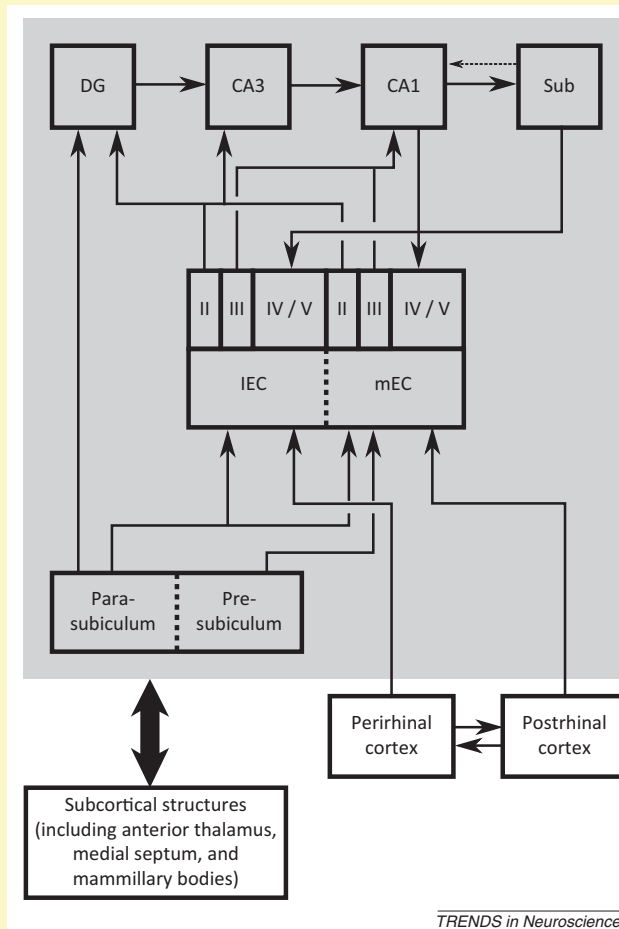
Figure 1. Anatomy of the hippocampal formation. Subcortical structures – including the medial septum, mammillary bodies, and anterior thalamus – project to all subfields of the hippocampal formation, most notably via the fimbria/fornix fibre bundle. Post- and perirhinal cortices provide neocortical input to medial entorhinal cortex (mEC) and lateral entorhinal cortex (IEC), respectively. The presubiculum projects to mEC, whereas the parasubiculum projects to mEC, IEC, and dentate gyrus (DG). Both mEC and IEC provide input to the DG, CA3, and CA1 subfields of the hippocampus proper via the perforant path. Within the hippocampus proper, DG sends mossy fibre projections to CA3, CA3 sends Schaffer collateral projections to CA1, and CA1 sends output projections to the deep layers of mEC and IEC both directly and via the subiculum.
