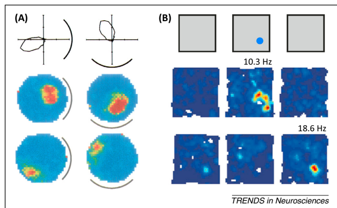
Figure 4. Other spatially receptive cell types of the hippocampal formation. (A) Head direction cells of the anterior thalamus. Head direction cell firing is not spatially modulated but strongly dependent on the animal's head direction in the horizontal plane. Top row: polar plots illustrate the directionally tuned activity of a single head direction cell recorded in a familiar environment, and how the preferred direction of that cell rotates with a distal visual cue (marked by a black line). Bottom rows: simultaneously recorded place cell responses illustrate how place field firing locations rotate coherently with the preferred orientation of head direction cells (reproduced, with permission, from [53]). (B) Object and object trace cells of the lateral entorhinal cortex. Top row: three recording sessions were performed in a familiar environment, with an object (marked by the blue dot) placed into the environment for the second session but removed for the third. Middle row: firing rate map of a typical object cell, which encodes the location of the object when it is present within the environment. Bottom row: firing rate map of a typical object trace cell, which encodes the previous position of objects that are no longer present within the environment (adapted, with permission, from [100]).
