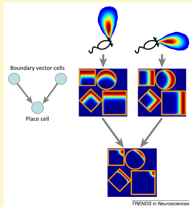
Figure 1. The boundary vector cell (BVC) model of place cell firing. Place cell firing patterns can be modelled as the thresholded sum of BVC inputs, which are tuned to respond to the presence of environmental boundaries at a fixed distance and allocentric direction from the animal. Putative firing rate maps are shown for two BVC inputs and a single place field output in four environments (adapted from [27]).
