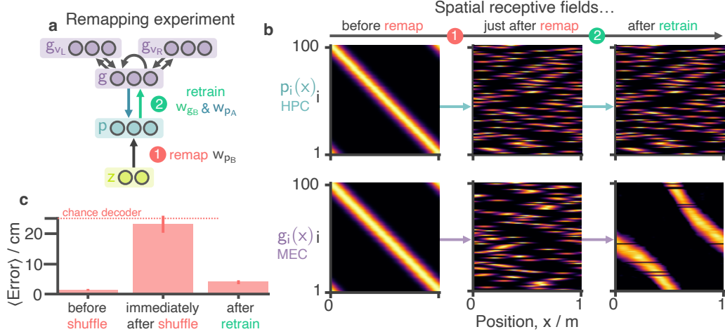
Figure 4: Remapping and transfer of structural knowledge between environments. a After training (as in Fig. 2) place cell inputs are shuffled to simulate a “remapping” event observed when an agent moves to a new environment. The agent then retrain for an additional 30 minutes; during this period internal MEC weights, and weights from the conjunctive cells to MEC are held fixed while MEC \leftrightarrow HPC weights remain plastic. b Receptive fields of the HPC and MEC neuronal populations at different stages in the experiment: Initially after remapping HPC and MEC inputs are randomised. MEC relearns rate maps as they were before remapping but with a constant phase shift. Note: neurons are ordered by the position of their peak activity on the track before remapping and this ordering is maintained in subsequent panels. c The error ( \pm SEM over 50 trials) after 1 second of path integration is shown at different stages of the experiment. Although path integration is initially disrupted after remapping it recovers despite no relearning of the MEC synapses where the ring attractor is stored.
