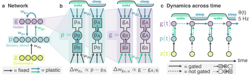
Figure 1: A biologically plausible generative model is trained with theta frequency wake-sleep cycles and a local learning rule. a Network schematic: high-D stimuli from an underlying environmental latent, z , arrive at the basal dendrites of the sensory layer, p , and map to the hidden layer, g (this is the inference model, weights in green). Simultaneously, top-down predictions from the hidden layer g arrive at the apical dendrites of p (this is the generative model, weights in blue). b Neurons in layers p and g have three compartments. A fast oscillation, \theta(t) , gates which dendritic compartment – basal ( p_B , g_B ) or apical ( p_A , g_A ) – drives the soma. A local learning rule adjusts input weights to minimise the prediction error between dendritic compartments and the soma. c This equates to rapidly switching “wake” and “sleep” cycles which train the generative and inference models. Panel c displays just two updates per theta-cycle, in reality there are many ( \delta t \ll T_\theta ).
