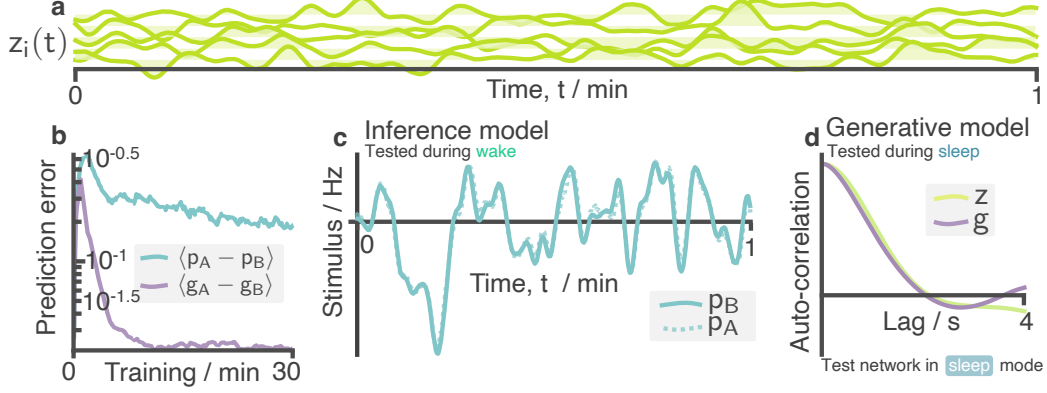
Figure 2: Learning in an environment of temporally varying latents. a In this artificial task the latent space comprises of N_z = 5 independent random variables with an autocorrelation decay timescale of 1 s. b Prediction errors (difference between apical and basal activations) in sensory and hidden layers reduce over training time. c Tested in wake mode ( \theta = 1 ) after training, the ground truth stimulus matches apical prediction for all stimulus dimensions (one shown) implying the network is efficiently “autoencoding” the sensory inputs into and back out of the compressed hidden layer. d Tested in sleep mode ( \theta = 0 , no environmental inputs), generated data from the hidden units, g , have an autocorrelation curve which matches that of the true latents implying a statistically accurate generative model has been learned. More extensive samples from this model, before and after training, can be found in Fig. ??
