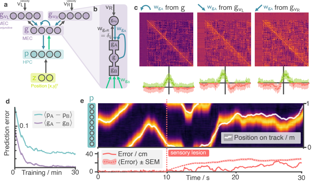
Figure 3: The hippocampal model learns to path integrate on a 1D track using a ring attractor. a Position selective (place cell) inputs drive basal dendrites of the sensory layer p (HPC). b Hidden units (MEC) are connected to two sets of “conjunctive cells” which each connect back to one of the hidden neurons ( g ) and either the leftward (for g_{vL} ) or rightward (for g_{vR} ) velocity of the agent allowing velocity information to enter the network. Synaptic strengths of the return connections from the conjunctive cells to the MEC hidden units, as well as those for the MEC recurrent connectivity (collective denoted w_{gA} ), are randomly initialised and plastic. c After training, reordering the hidden units by the position of peak activity reveals a ring attractor in the synaptic weight matrices. Centre-surround recurrent connectivity stabilises an activity bump which is then “pushed” around the attractor manifold by asymmetric connections from the conjunctive cells, integrating velocity. Bands of zero weights show MEC neurons which have become perpetually inactive (aka “died”). The bottom panel displays the matrix row-averages, utilizing the circular symmetry of the environment to align rows before averaging. d Learning plateaus after 15 mins of simulated time. e Path integration ability is demonstrated in a lesion study: after 10 seconds in the normal oscillatory mode the network is placed into sleep mode (aka generative mode), lesioning the position-dependent sensory inputs. Despite this HPC continues to accurately encode position, evidence that the MEC ring attractor is path integrating the velocity inputs and sending predictions back to HPC. Lower panel shows the accumulated decoding error as well as the mean \pm SEM over 50 trials.
