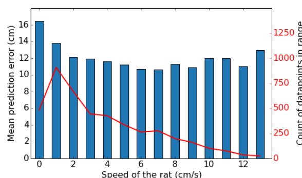
Fig 1. S1 Fig. Mean prediction error for different instantaneous movement speeds. Movement speed is based on the distance covered in 200 ms. The first bar is the average over the errors for speeds in range [0, 0.5] cm/s, the second for (0.5, 1.5] cm/s, etc. The error is highest when the rat is not moving or moving very slowly. Notice that speeds in the range of 1-2 cm/s can also be the results of head movements. At higher speeds the exact velocity does not seem to influence accuracy. Note that the bars do not contain the same amount of data points. Apparent changes in the mean error at higher velocities can be attributed to noise as we have less data points there.
