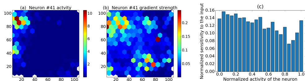
Fig 6. Gradient analysis: sensitivity decreases with activity. (a) Place field of an example neuron. (b) Sensitivity field - absolute values of gradients in different locations for the same neuron. (c) Normalized sensitivity as a function of normalized activity across neurons.
