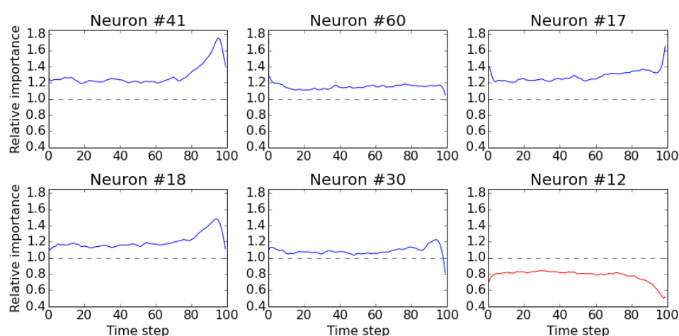
Fig 2. Gradient analysis. a-e) Temporal profiles of relative importance for 5 selected neurons among the highest contributing neurons according to gradient analysis. Notice that the profiles peak at different time steps. f) Temporal profile of the least important neuron according to gradient analysis.
